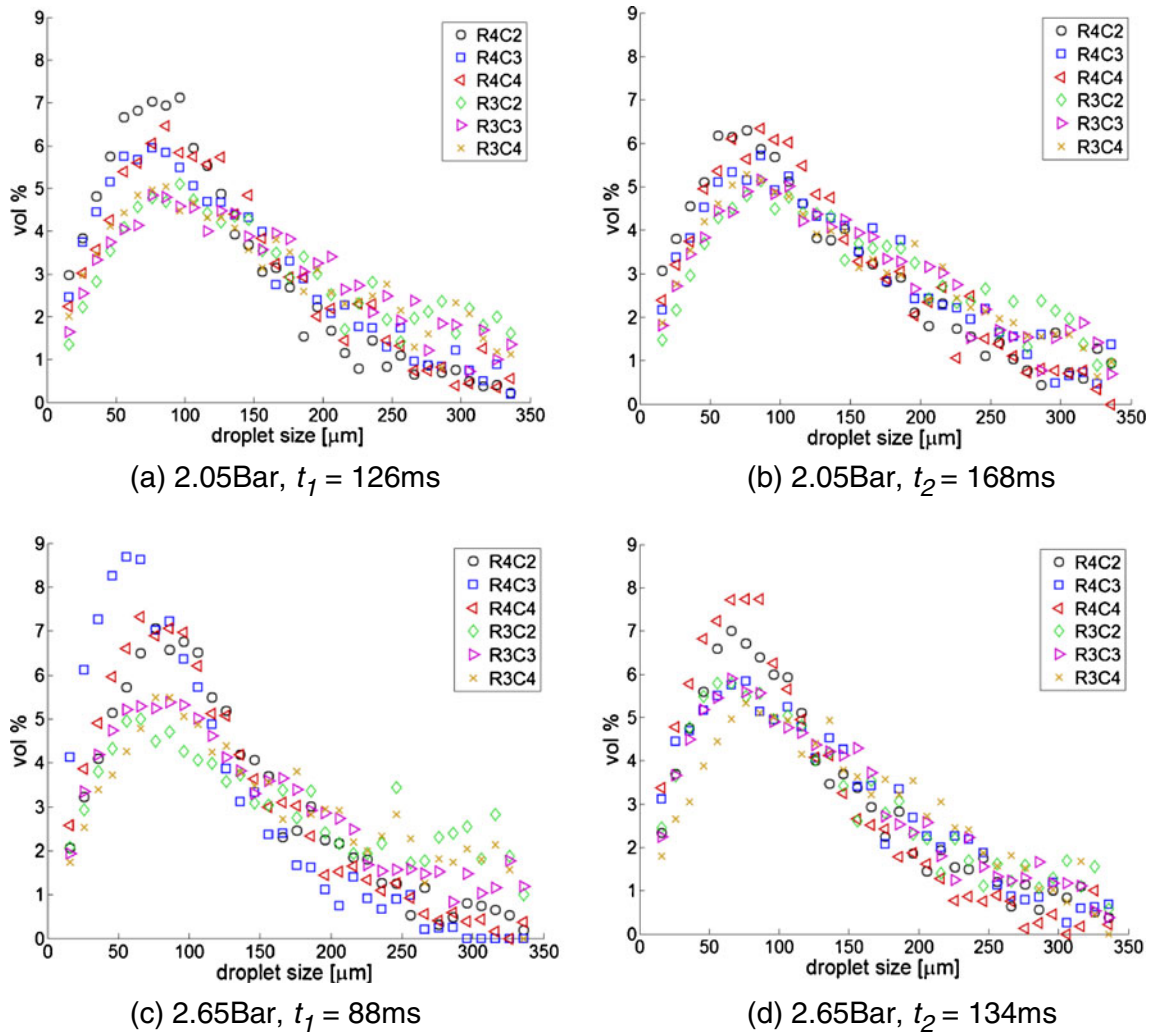
Fig. 7 Droplet size distributions of the volume mean diameters obtained for six FOVs along the rows R3, and R4 at (a) 2.05Bar, t_1=126 ms (b) 2.05Bar, t_2=168 ms, (c) 2.65Bar, t_1=88 ms and (d) 2.65Bar, t_2=134 ms.
