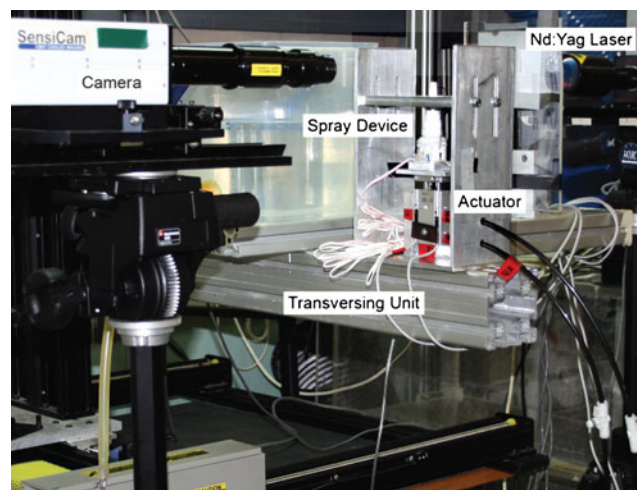
Fig. 2 Experimental setup of the high speed photography using a Particle/Droplet Image Analyser system.
